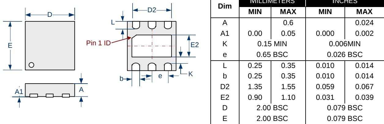
Figure 13 · LU 6-Pin Plastic UDFN 2mm x 2mm x 0.6mm Package Dimensions
