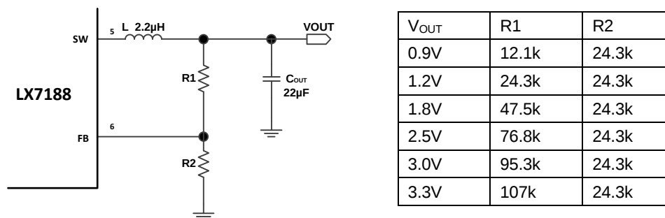
Figure 12 · Output Circuit
