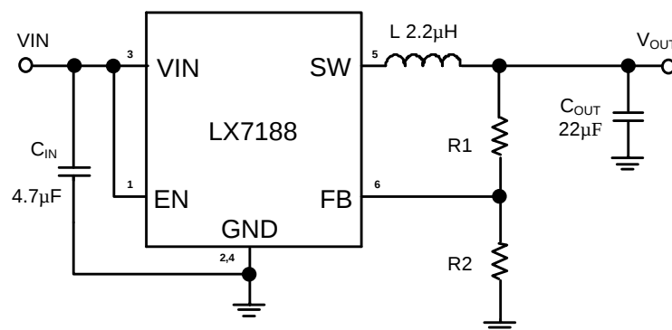
Figure 11 · Typical Application
